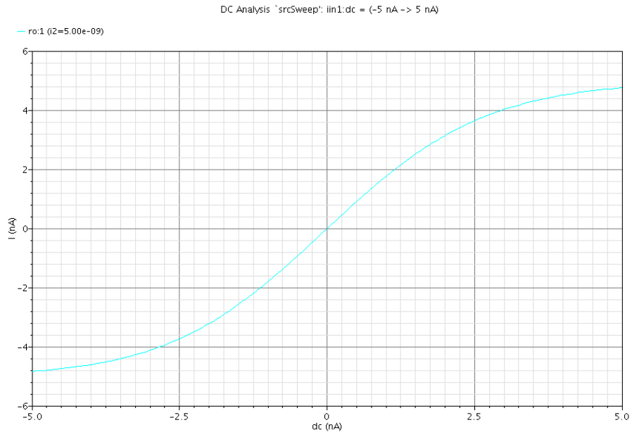
Figure 6. DC transfer characteristics of the sigmoidal circuit
