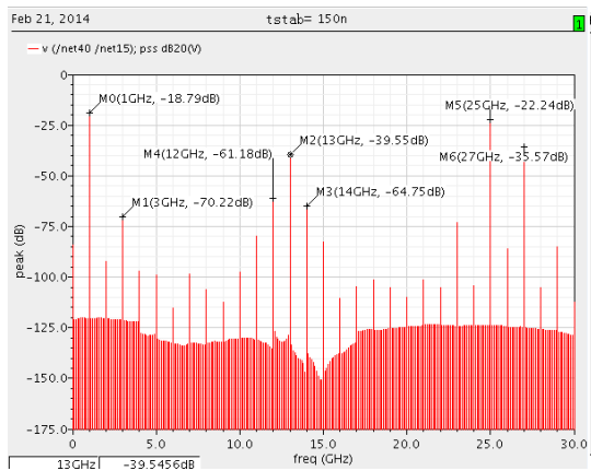
Fig.4 tatab=150ns, spectrum result from PSS
