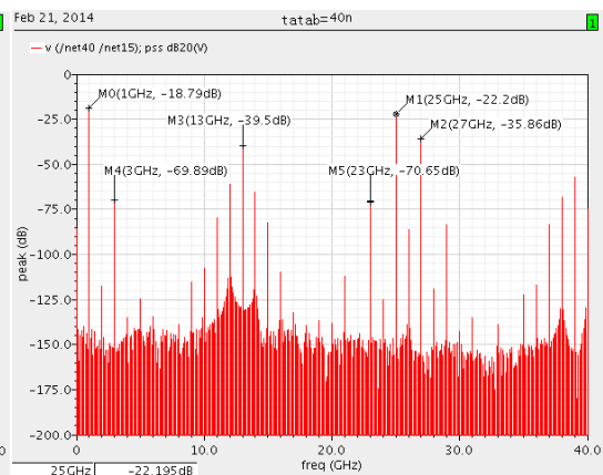
Fig.3 tatab=40ns, spectrum result from PSS
