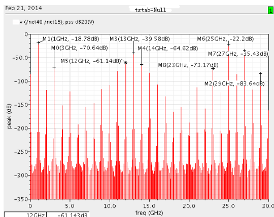
Fig.2 tstab=NULL, spectrum result from PSS
