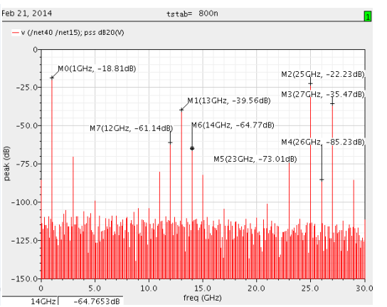
Fig.5 tatab=800ns, spectrum result from PSS
