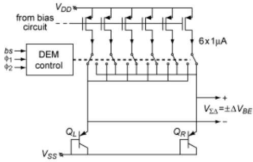
Fig. 7. Current-source configuration used to obtain a dynamically matched 1:5 bias current ratio for generating \Delta V_{BE} .
