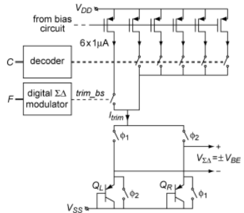
Fig. 8. Current-source configuration used to obtain a trimmable bias current I_{trim} for generating V_{BE} .
