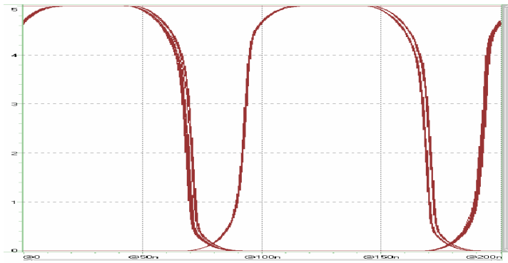
Figure 2 Eyediagram2
