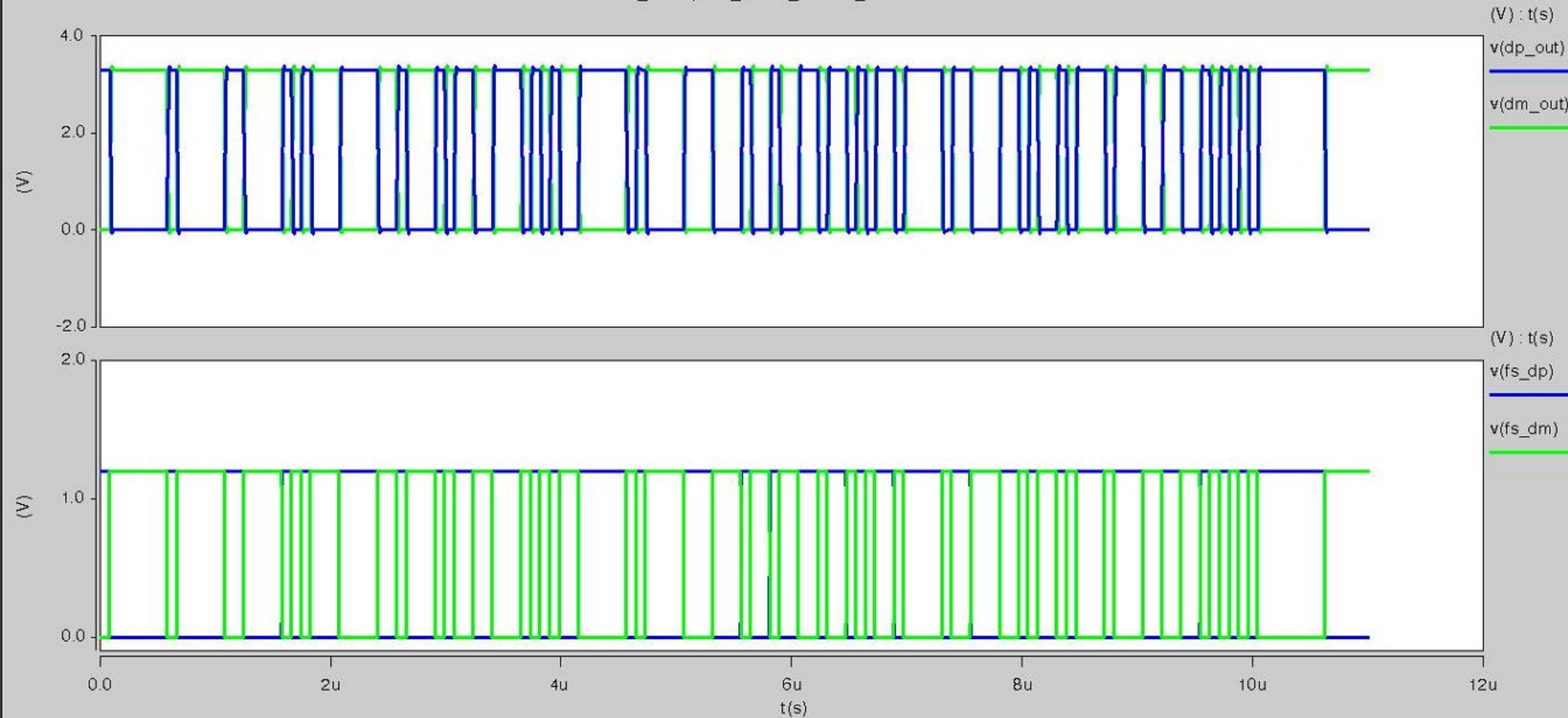
USB_Full Speed_PRBS_127bits_BitTime83nSec
