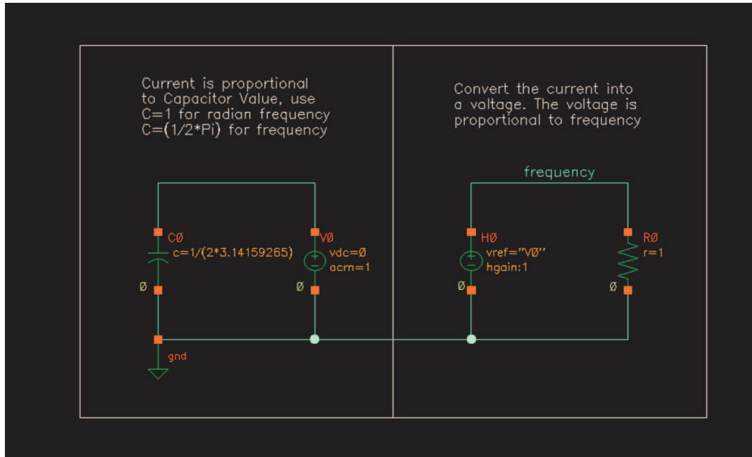
Circuit to generate frequency
