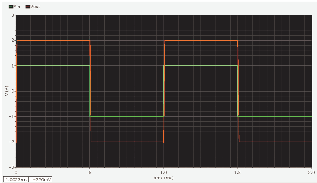
Figure 2: Transient Response of the Current Gain Testbench
