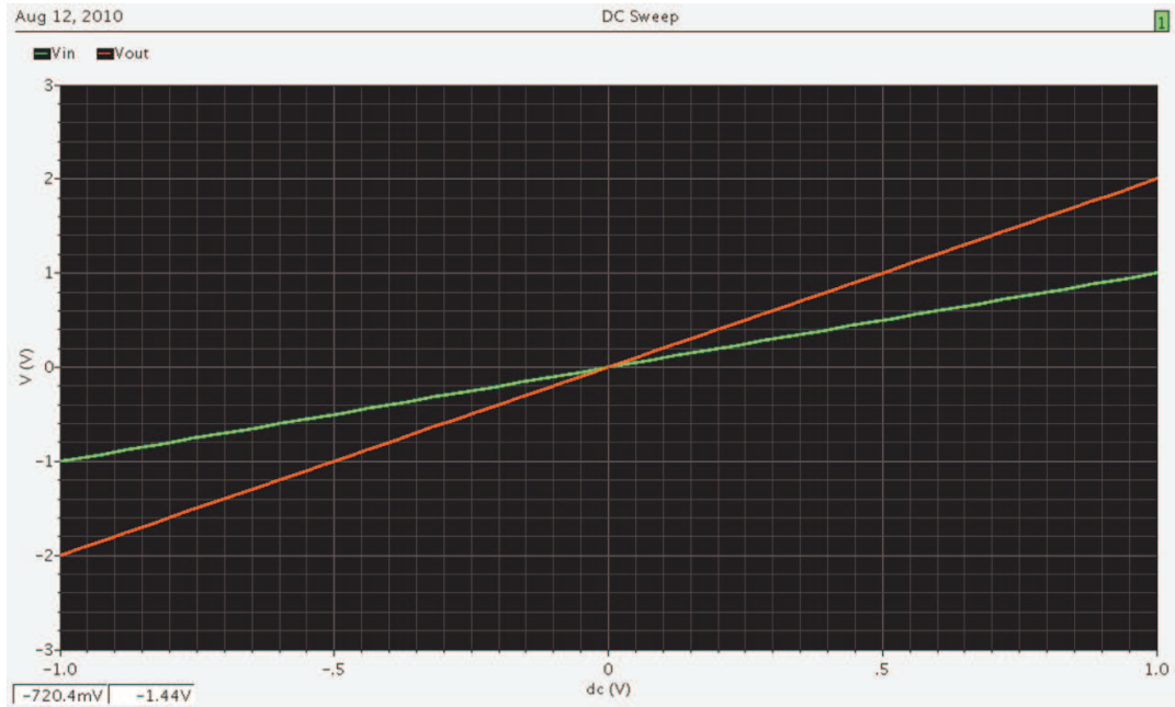
Figure 1: DC Sweep Results for Current Gain Testbench
