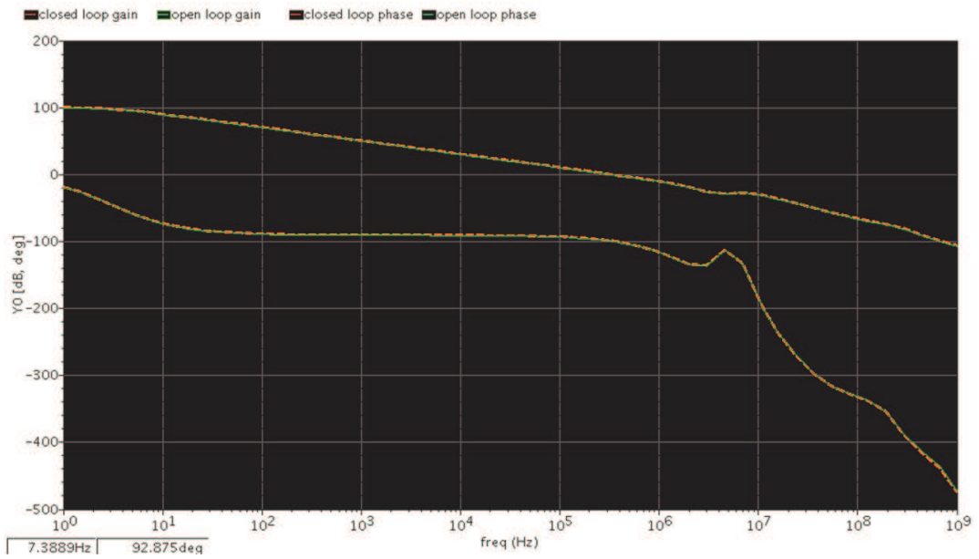
Figure 2: Comparison of Closed Loop and Open Loop Simulation Results
