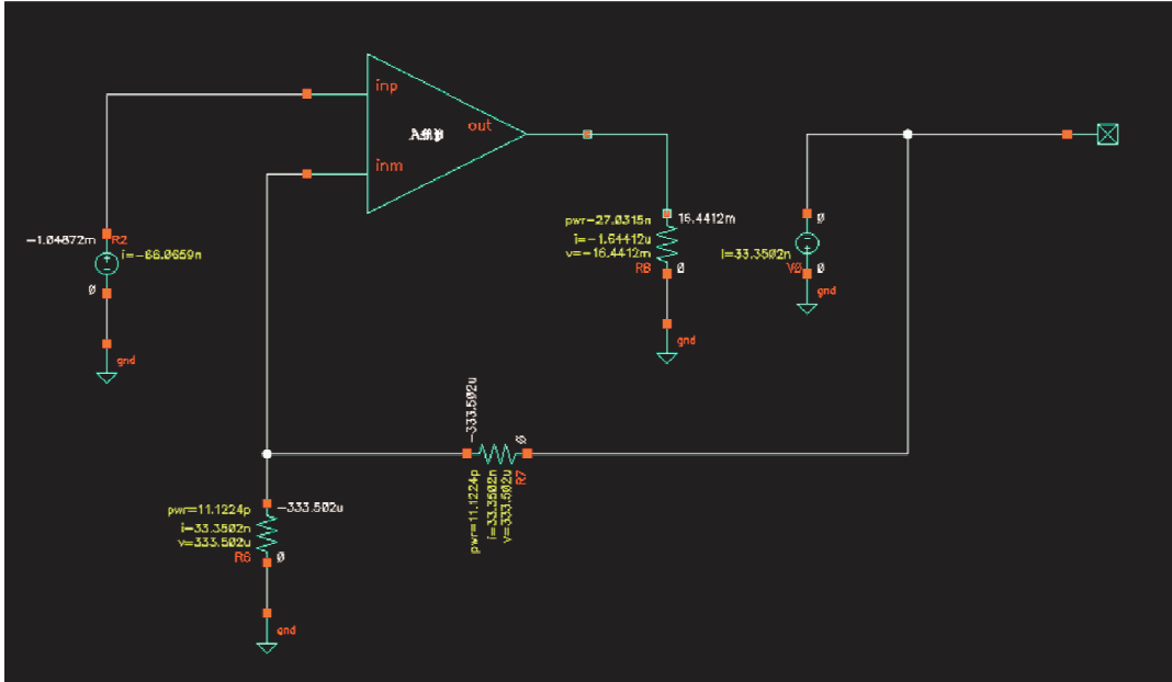
Figure 1: Open Loop Testbench
