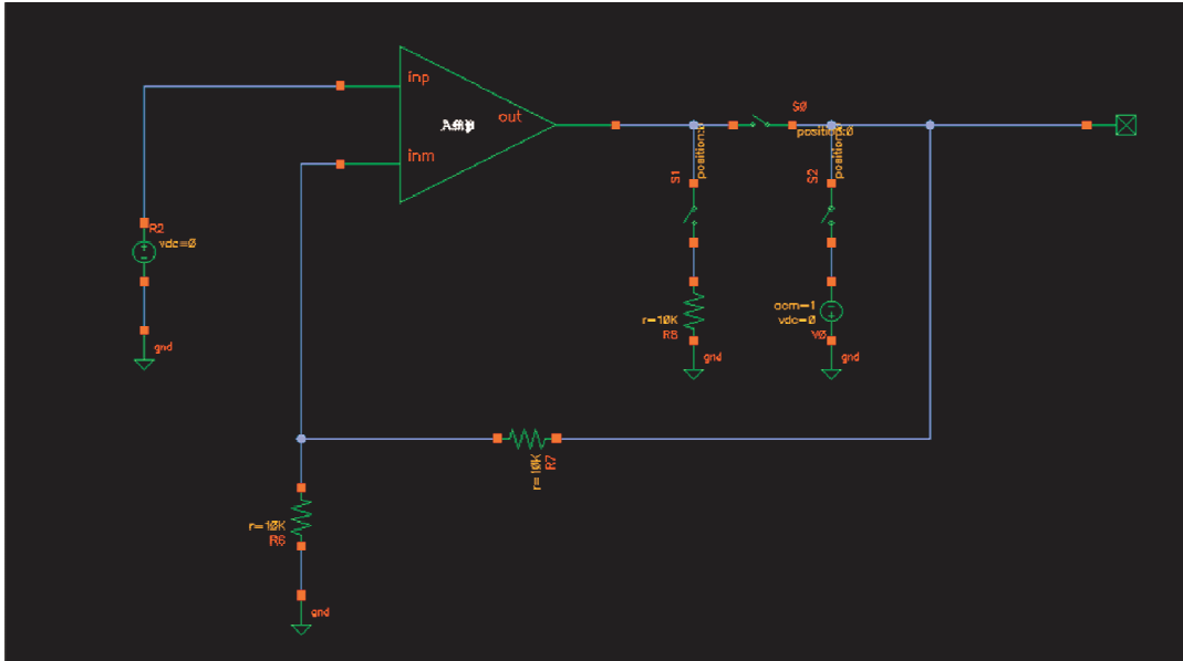
Figure 1: Modified Open Loop [Switch] Testbench
