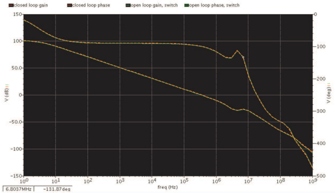
Figure 2: Comparison Open Loop [Switch] and Closed Loop Simulation Results
